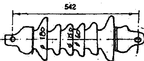
(ii) 9 TONNE INSULATOR
