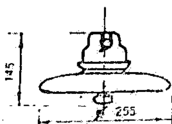
(v) 10" DISC INSULATOR
