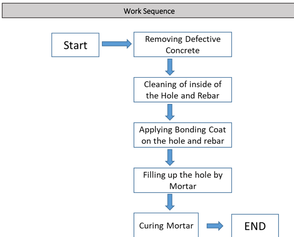
Figure: 1.3 Work sequence of Hand applied mortar
