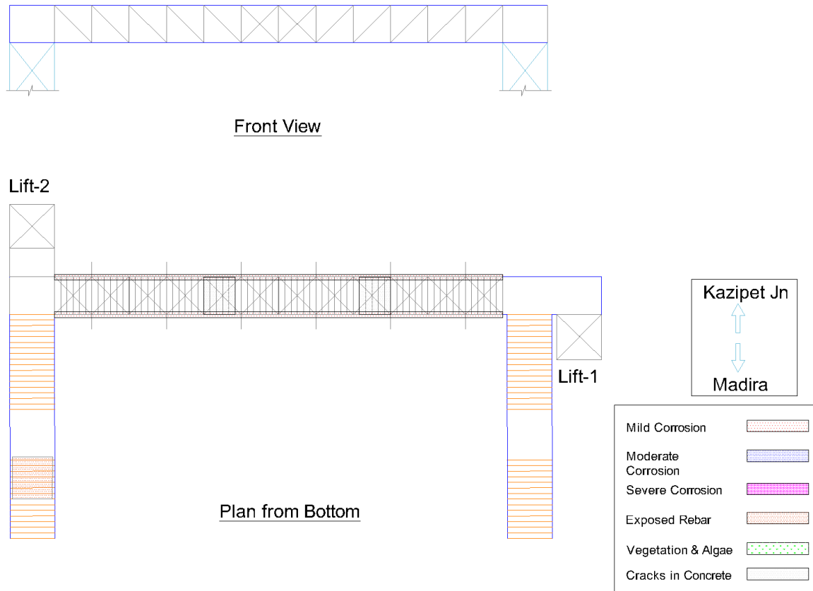
Fig 2.1: Locations of Deteriorations in span 1
