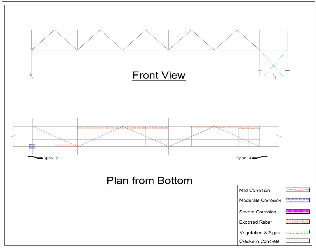
Fig: 3.7 Locations of deteriorations and bottom view of span-3
