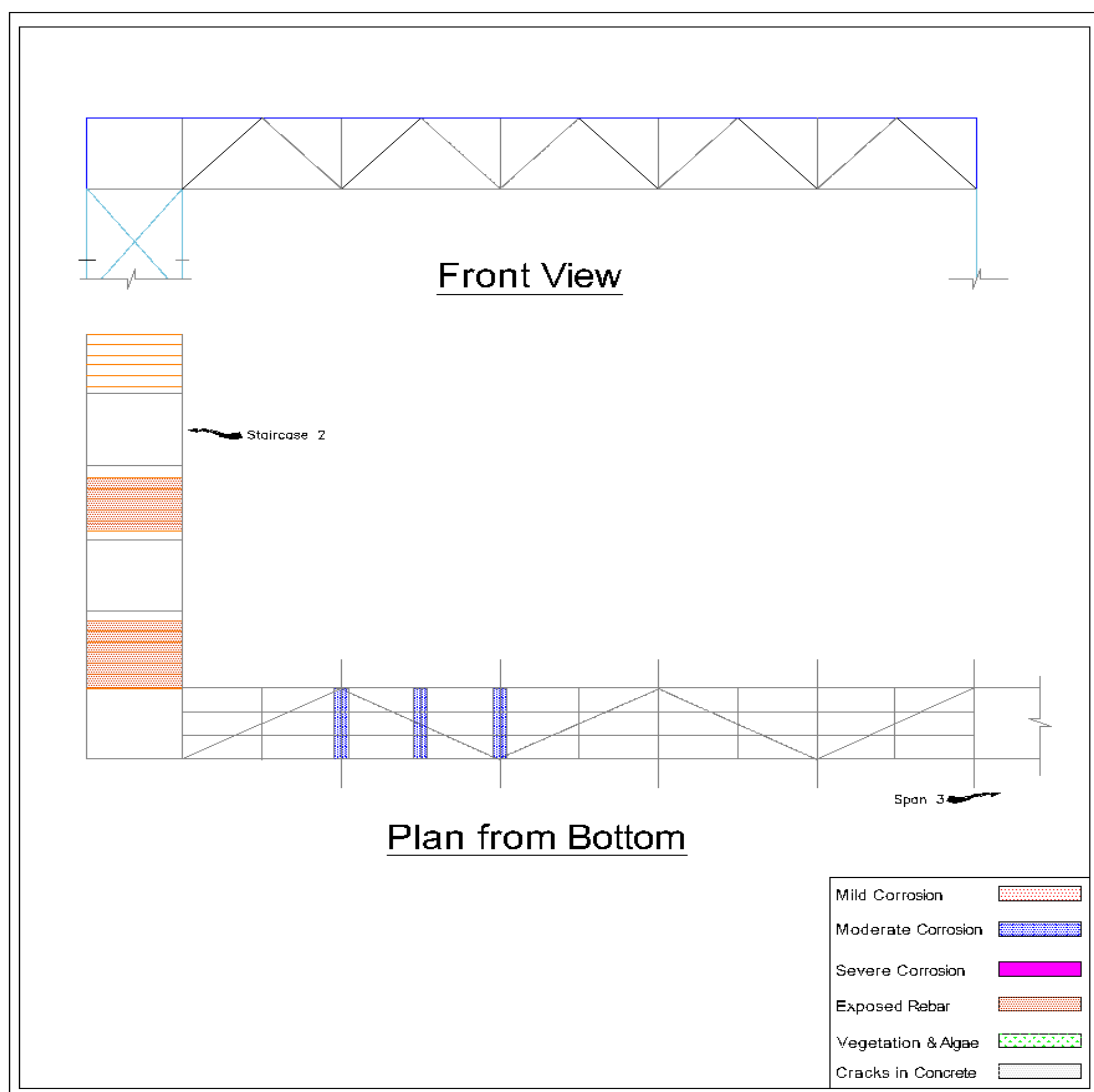
Fig: 3.4 Locations of deteriorations and bottom view of span-2
