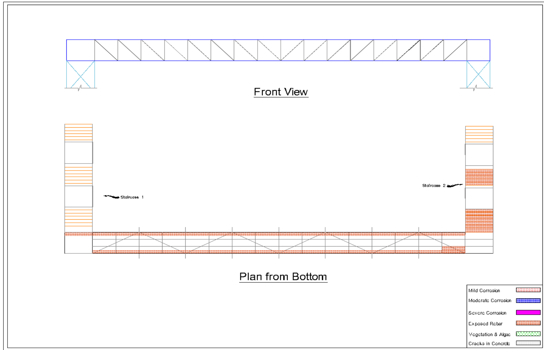
Fig 3.1: Locations of deteriorations and bottom view of Span-1
