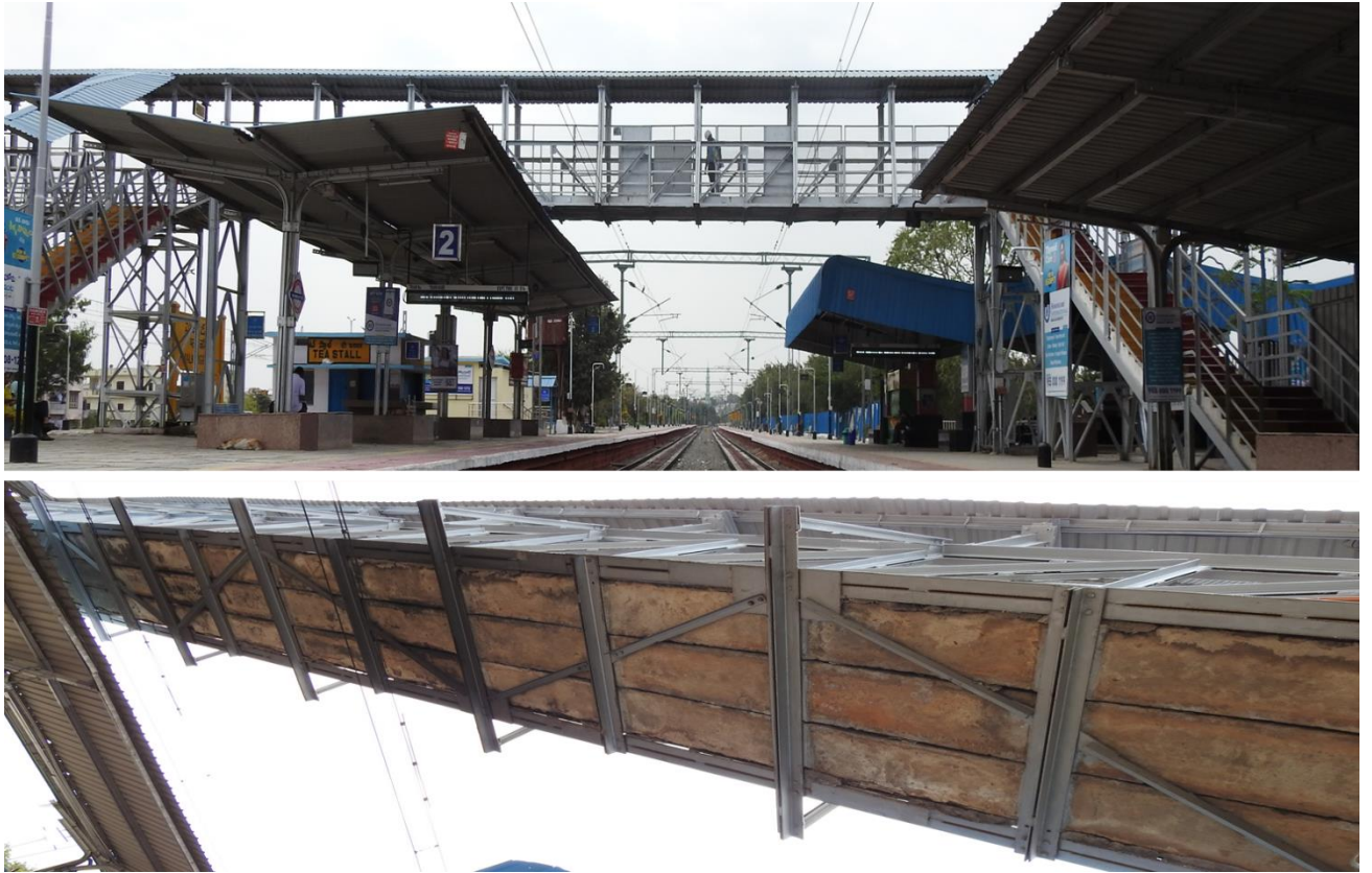
Fig 1.3: Front view and bottom view of span 1
